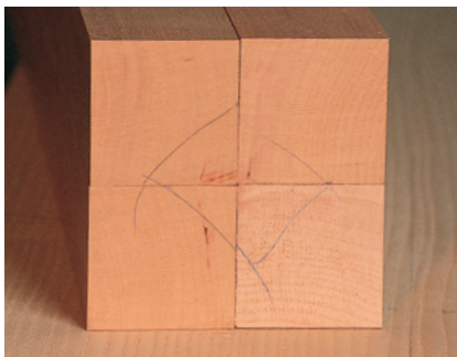
The diamond marked on the tops of the four legs will always allow you to recognize the inside and outside faces of the legs.
