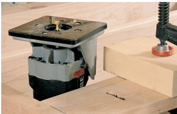
A keyhole bit fitted in a hand-held router and run along a guide block is an easy way to attach the shelf to a wall
