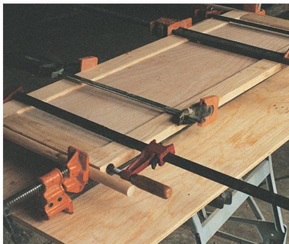
The lid is a simple frame-and-panel assembled with biscuits and glue. But because the panel is a piece of plywood, you don't need to worry about seasonal expansion or contraction.
