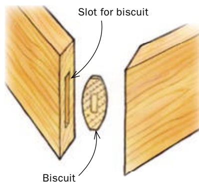
BISCUITED MITER
