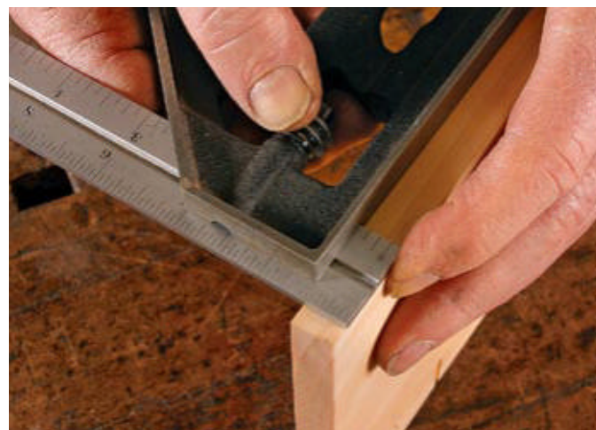
A thickness gauge. Adjust the ruler to match the thickness in one corner, then compare at the other three to see if the stock is consistently thick. Your fingertip will feel the slightest difference.
