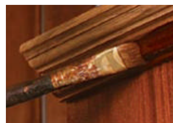
Seal the wood. Go over the surface a couple of times with a pad to apply a thin coat of shellac. Keep the pressure light to avoid filling the pores. It is easier to get into corners, carvings, and moldings by applying the shellac with an artist's brush (above).
