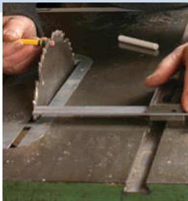
Check sawblade and miter slot for parallel. Use the inside edge of the miter slot as a reference surface and adjust the table if necessary.
