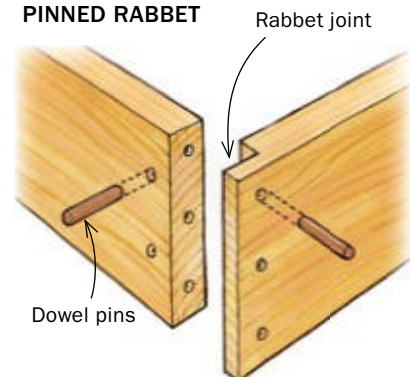
PINNED RABBET
